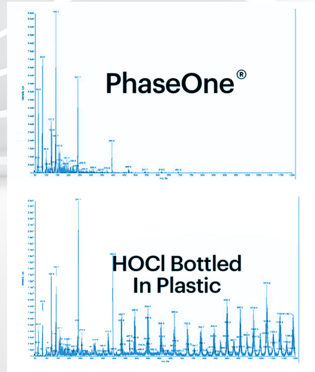
MASS SPECTROSCOPY 3 PHASEONE VS. EXAMPLE OF HOCl BOTTLED IN PLASTIC.
